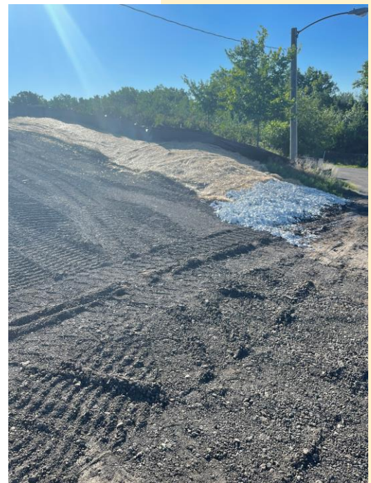
Riprap, asphalt grindings, and silt fence make for a sturdier route for disposal of earth on the landfill.
