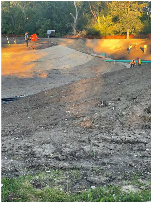
Turf reinforcement mat, topsoil, and seed were placed on the slopes of the new Par 3 Storage Facility.
