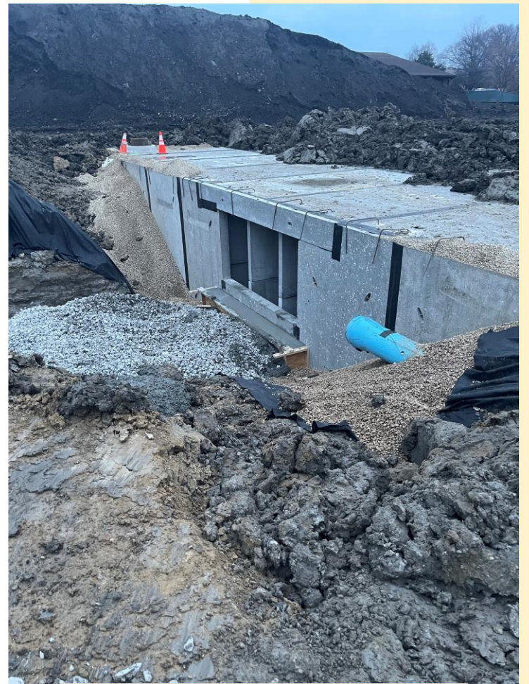
Little Duke will then be connected to the Par 3 Storage Facility via large box culverts
