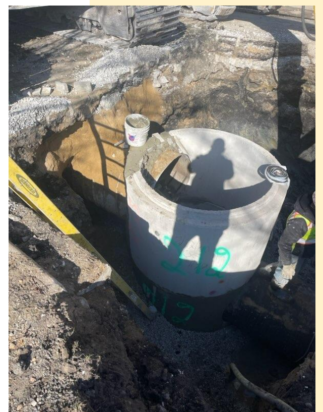
Connection of existing storm sewer to the box sewer on Hibbard
